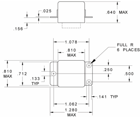
MOUNTING STYLE D
