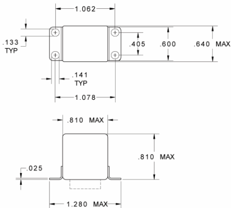
MOUNTING STYLE J
